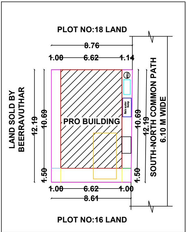
SITE PLAN & KEY PLAN
