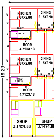
PRO., GROUND FLOOR PLAN
