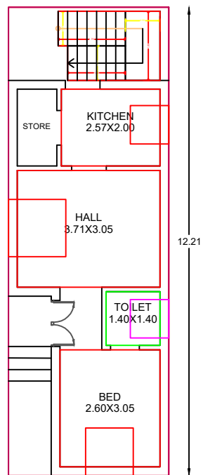
PROPOSED GROUND FLOOR PLAN
