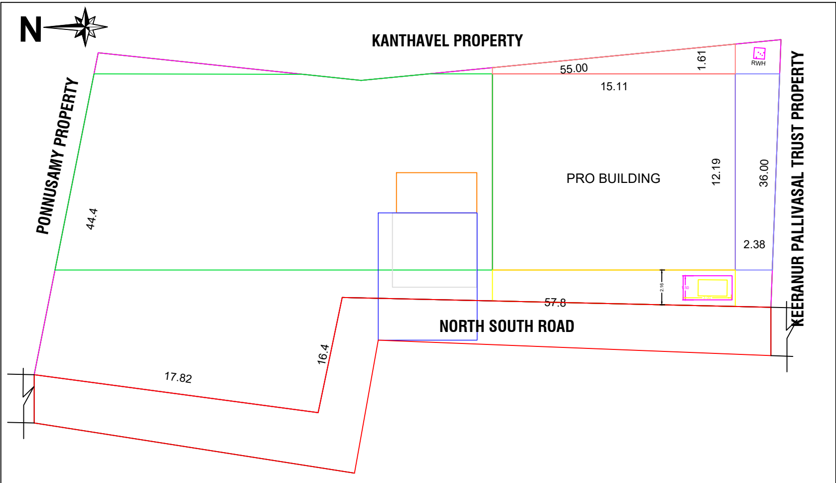
SITE PLAN
