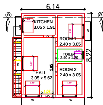
PROPOSED GROUND FLOOR
