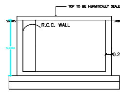
RWH_CAPACITY_L=5000LTRS
