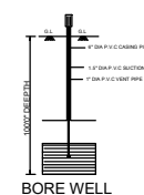
BORE WELL
