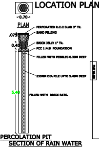
PERCOLATION PIT SECTION OF RAIN WATER
