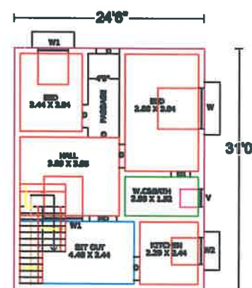
EXIST.GROUND FLOOR PLAN
