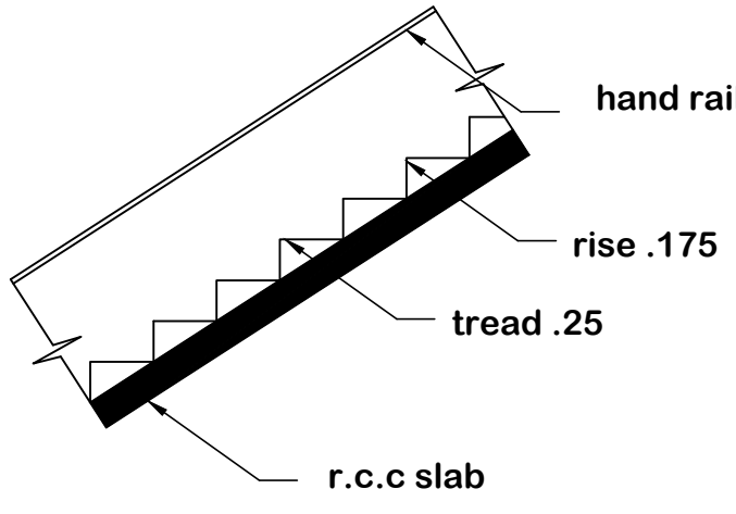
STAIR
