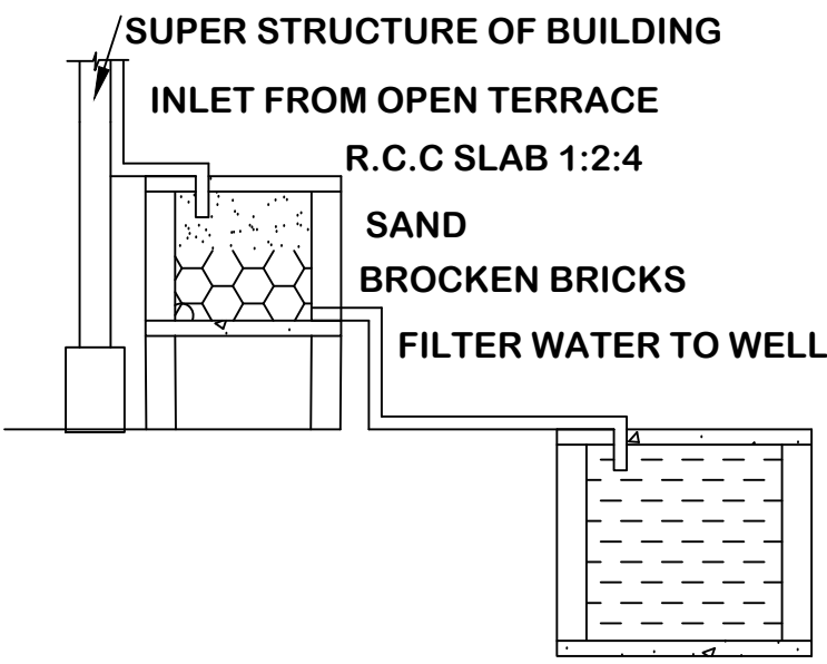
RAINWATER HARVESTING
