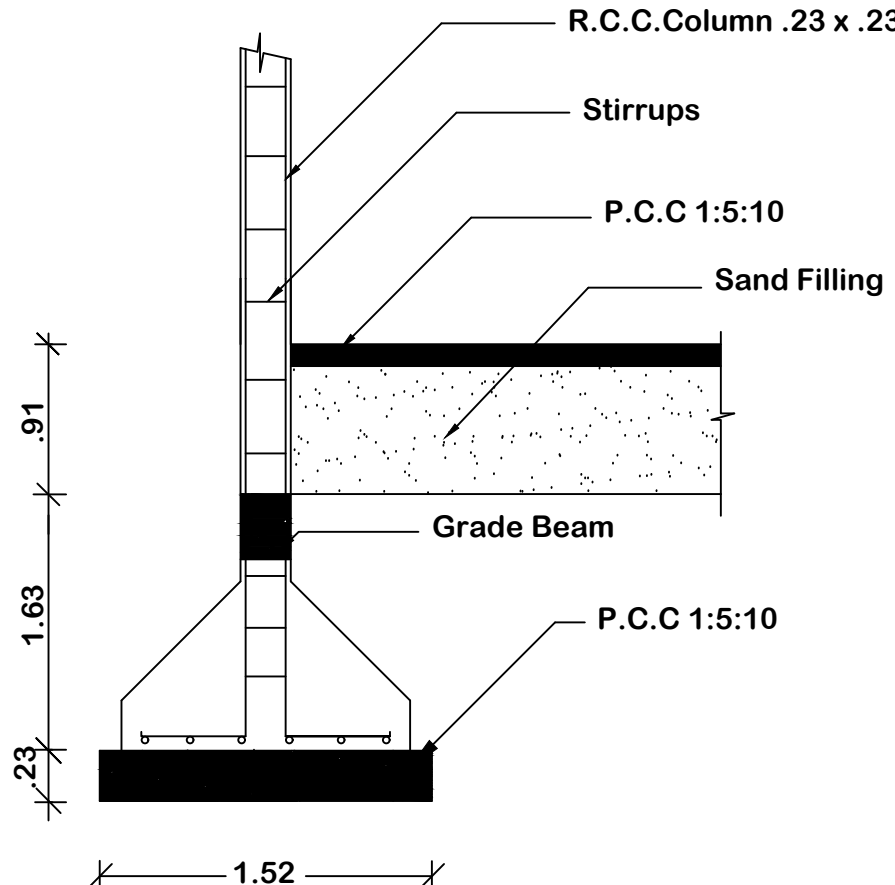
COLUMN DETAIL
