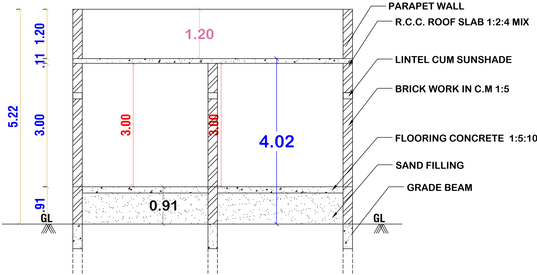
SECTION-"AA"
