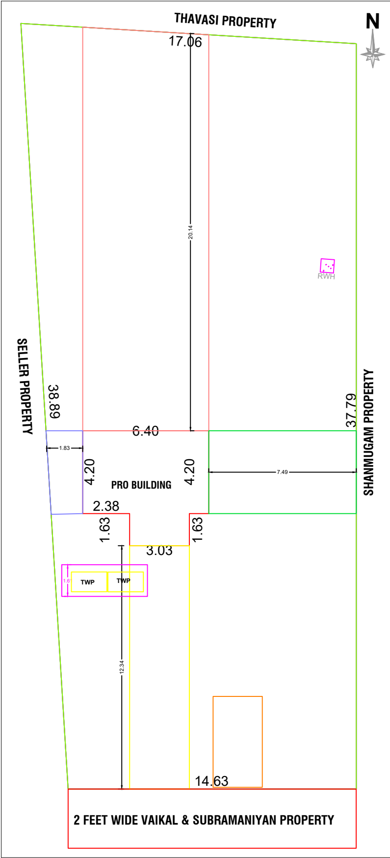
SITE PLAN
