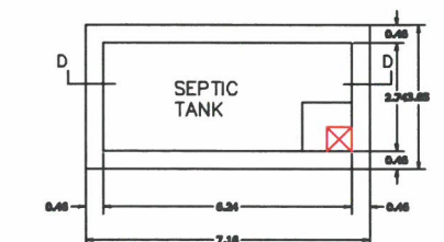
PLAN OF SEPTIC TANK SCALE 1"=2'-0"
