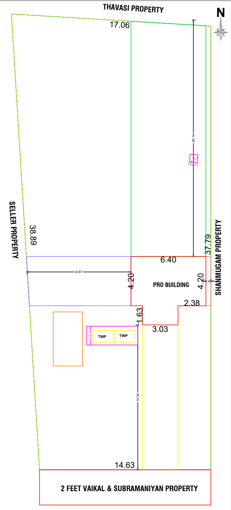
SITE PLAN
