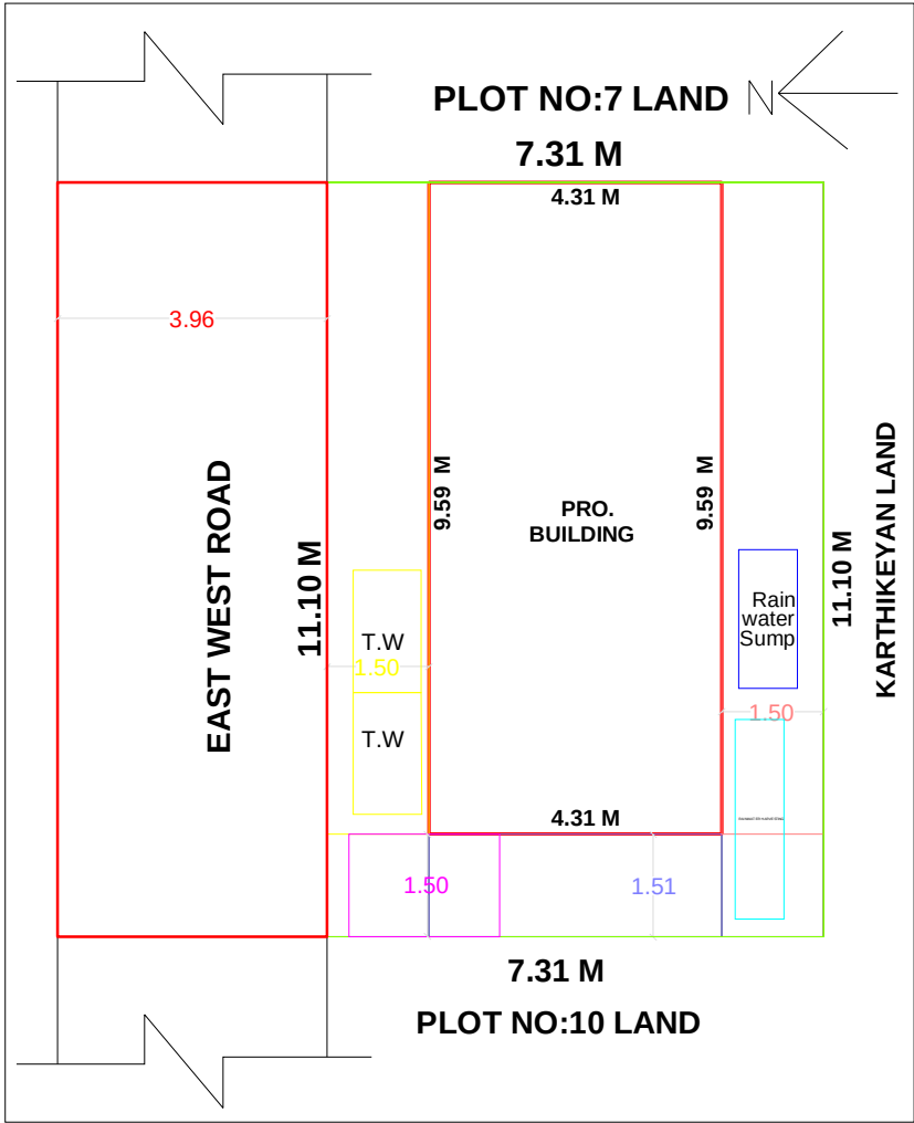
SITE FLOOR PLAN PROPOSED
