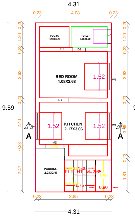
GROUND FLOOR PLAN PROPOSED
