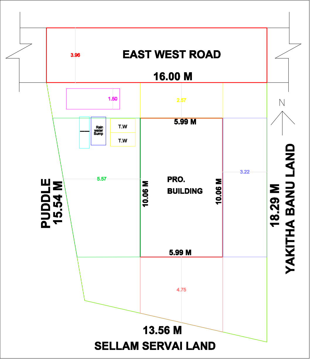
SITE FLOOR PLAN
