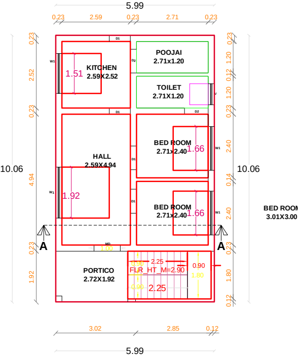
GROUND FLOOR PLAN PROPOSED
