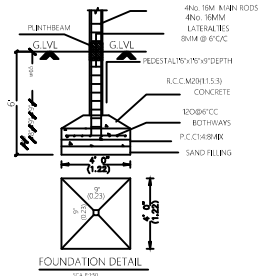
FOUNDATION DETAIL
