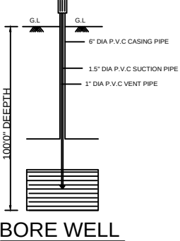
BORE WELL
