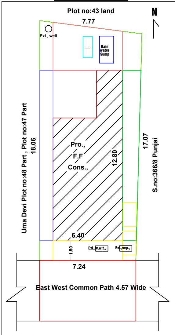
SITE PLAN & KEY PLAN (1:100)
