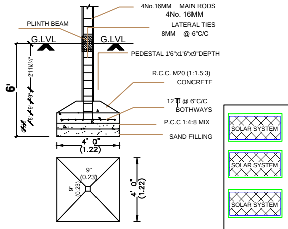
FOUNDATION DETAIL
