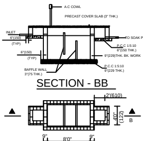
PLAN OF SEPTIC TANK
