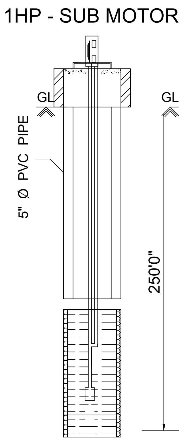
BOREWELL DETAILS
