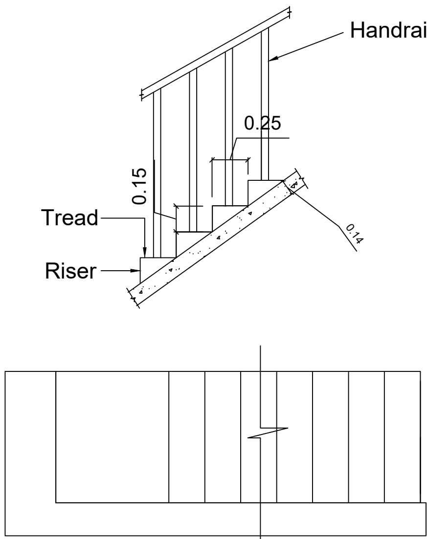
STAIRCASE DETAIL
