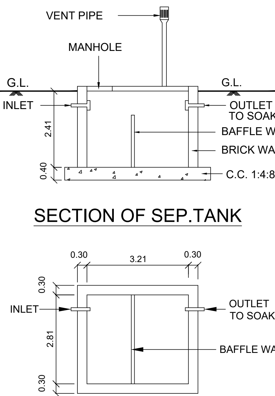
SEPTIC. TANK
