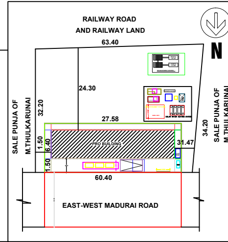
LOCATION & KEY PLAN
