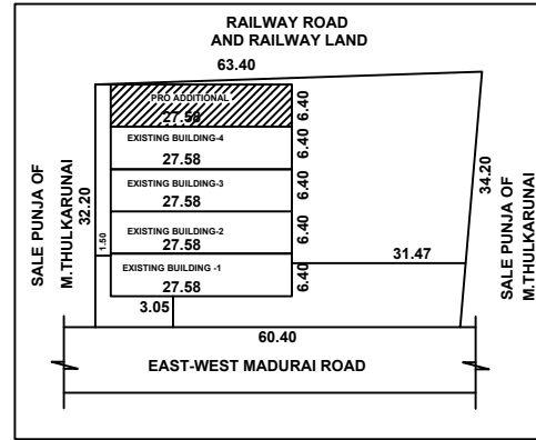
SITE PLAN
