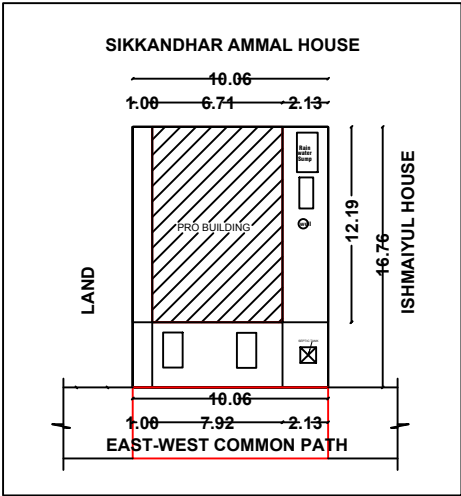
SITE PLAN & LOCATION PLAN
