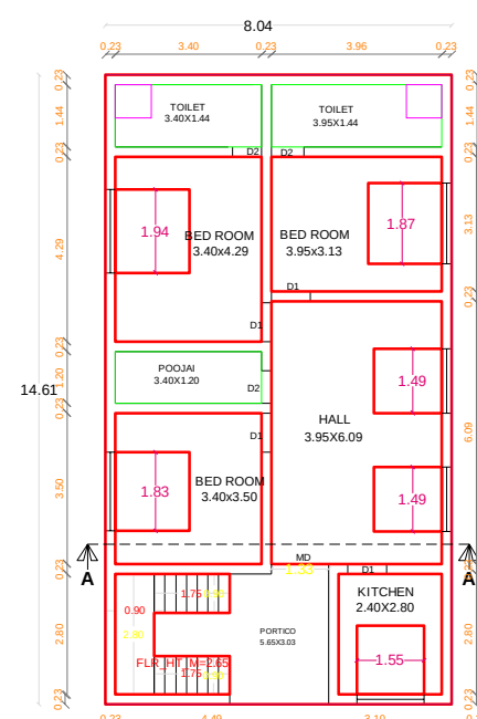
GROUND FLOOR PLAN PROPOSED
