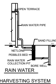
RAIN WATER HARVESTING SYSTEM
