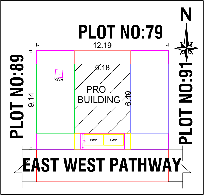
SITE PLAN
