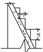
Staircase Detail Not To Scale
