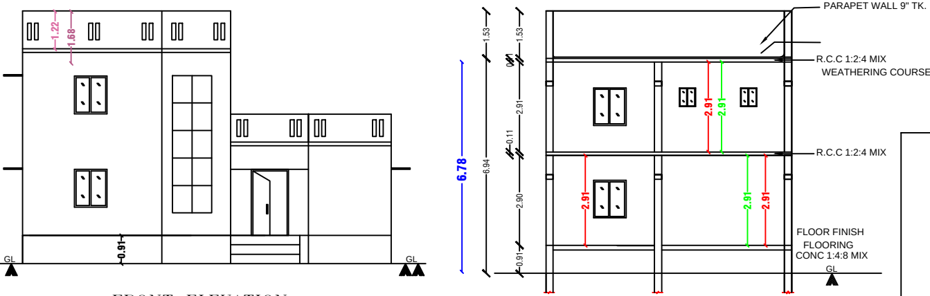
FRONT ELEVATION
