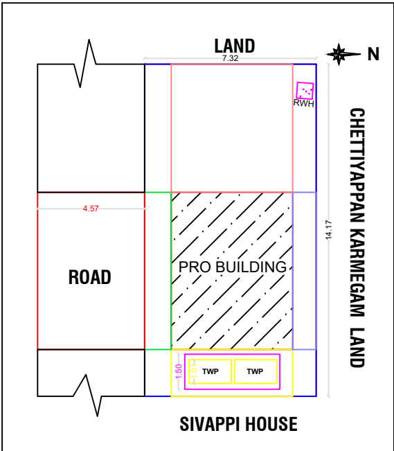
SITE PLAN
