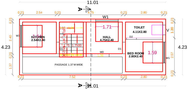
FIRST FLOOR PLAN PROPOSED
