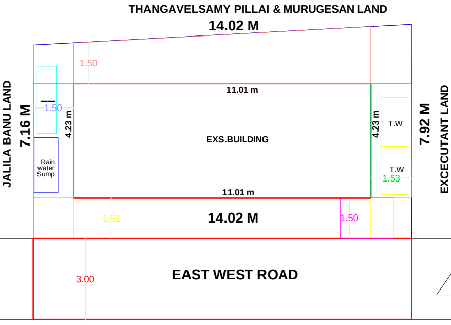
SITE FLOOR PLAN PROPOSED
