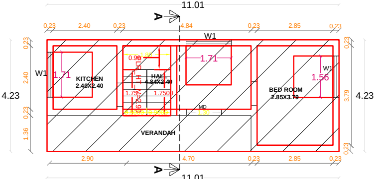
GROUND FLOOR PLAN EXISTING
