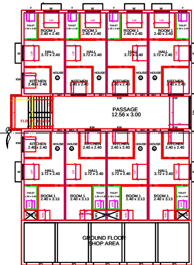
EXSITING GROUND FLOOR
