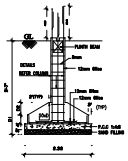
FOUNDATION DETAILS
