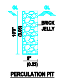
PERCOLATION PIT
