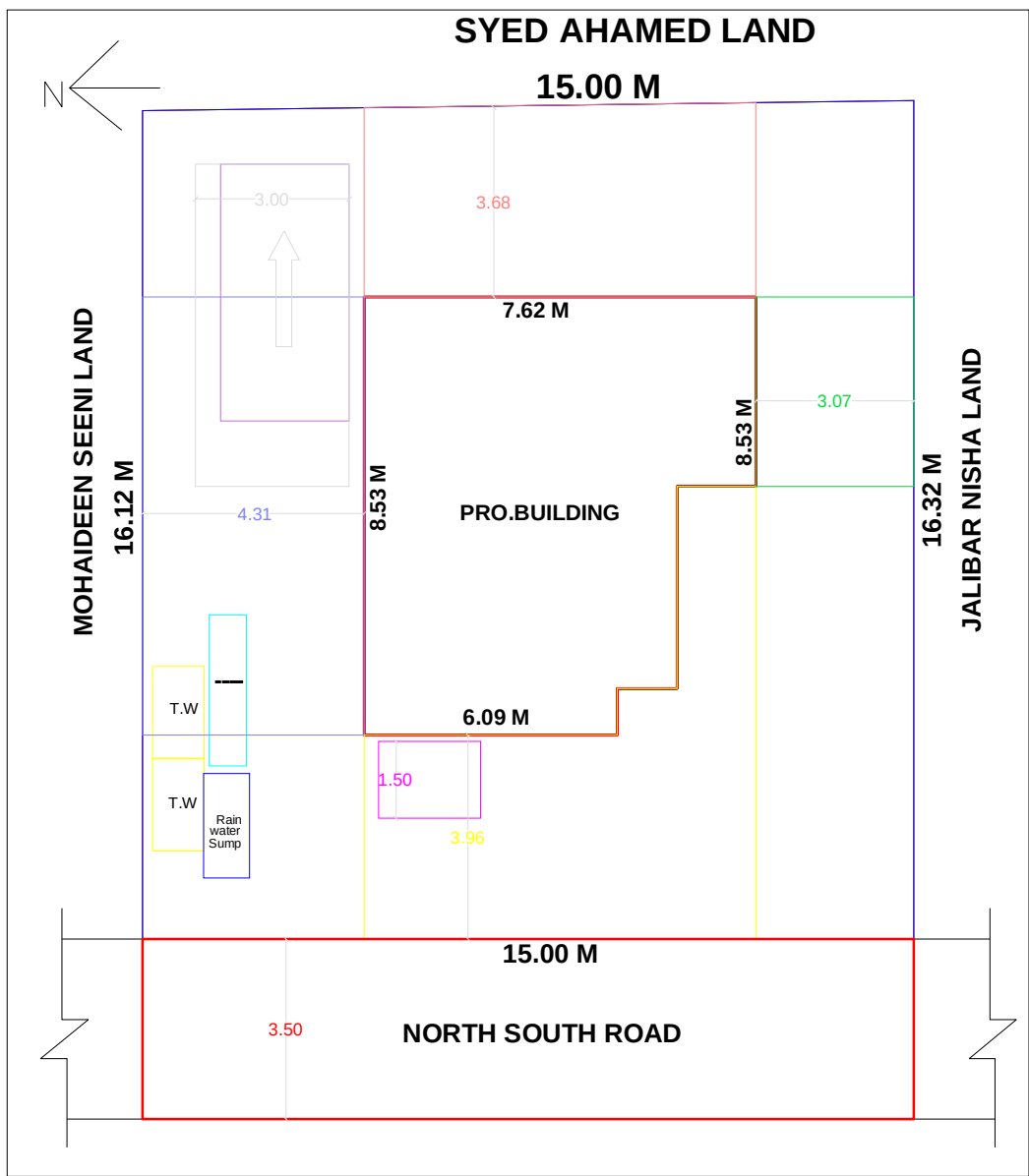
SITE FLOOR PLAN PROPOSED
