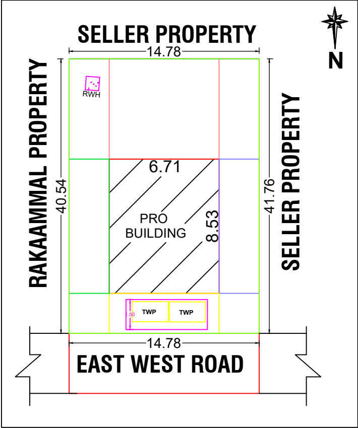
SITE PLAN
