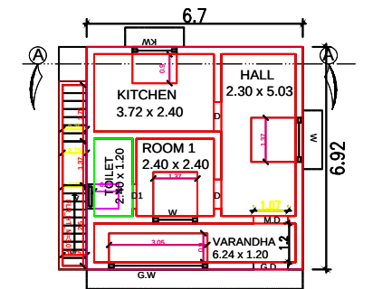
PROPOSED GROUND FLOOR
