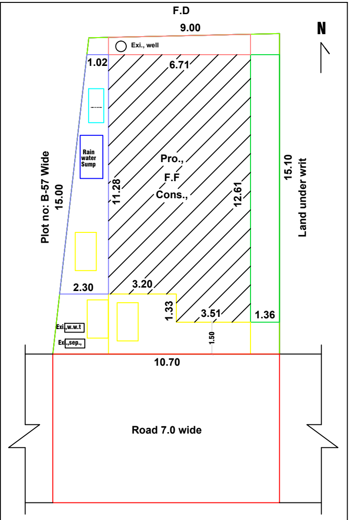
SITE PLAN & KEY PLAN (1:100)
