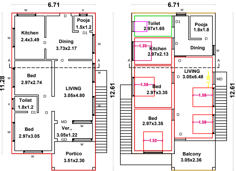
POSED FIRST FLOOR PLAN
