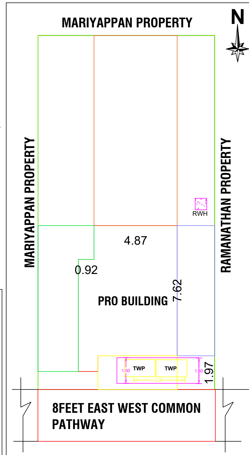
SITE PLAN
