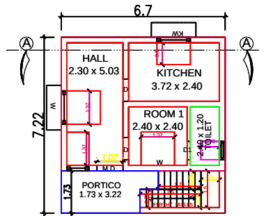
PROPOSED GROUND FLOOR
