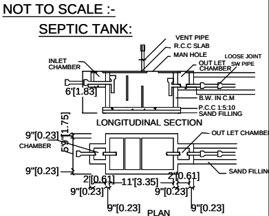
NOT TO SCALE :- SEPTIC TANK:
