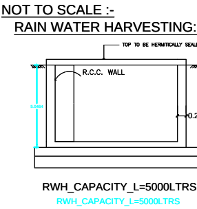
NOT TO SCALE :- RAIN WATER HARVESTING:
