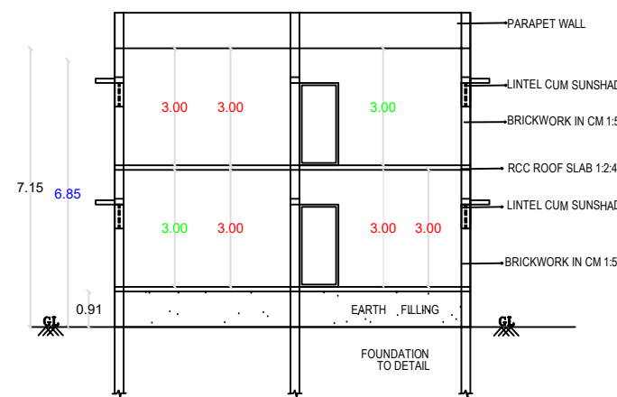
SECTION AB
