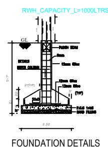
FOUNDATION DETAILS
