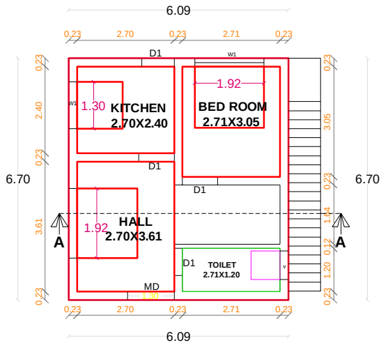
GROUND FLOOR PLAN PROPOSED
