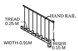
STAIRCASE DETAILS
