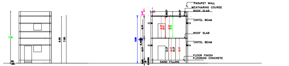
SECTION ON AB
