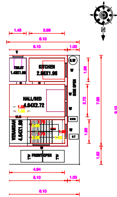
0. FIRST FLOOR PLAN
