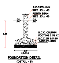
FOUNDATION DETAIL (DETAIL - B)
