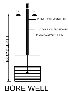
BORE WELL
