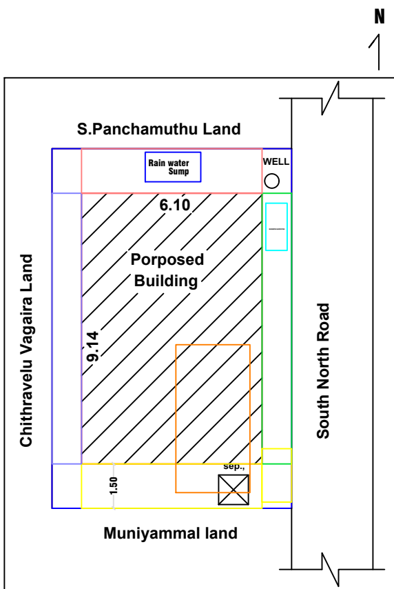
SITE PLAN CUM KEYPLAN
