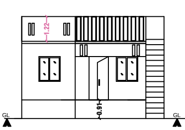
FRONT ELEVATION
