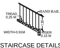
STAIRCASE DETAILS
