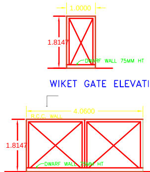
MAIN GATE ELEVATION
