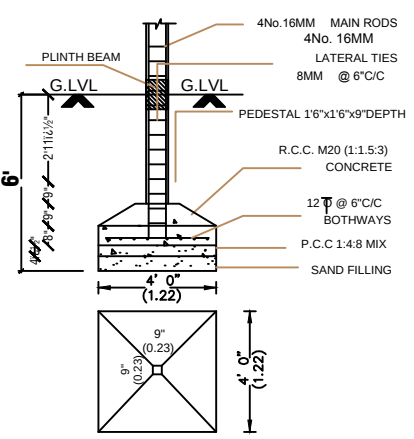
FOUNDATION DETAIL
