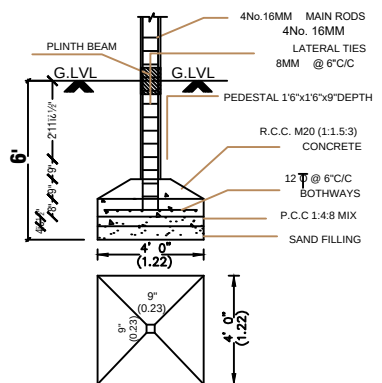
FOUNDATION DETAIL
