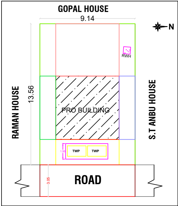
SITE PLAN
