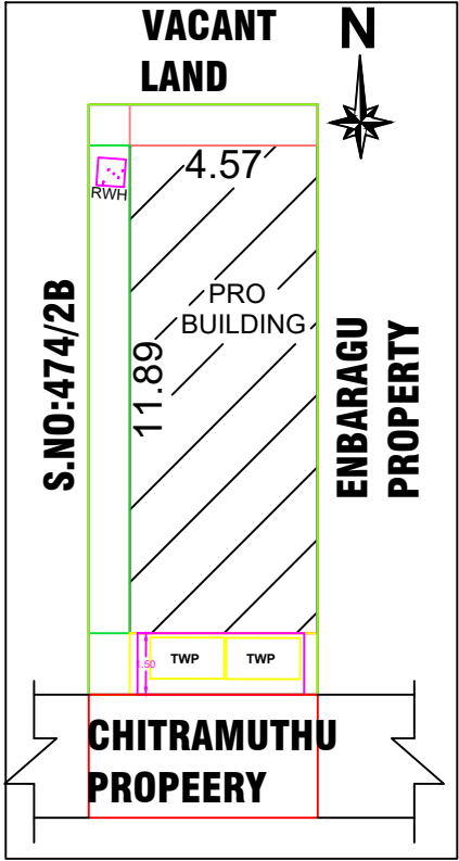
SITE PLAN
