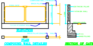
PLAN OF COMPOUND WALL DETAILS
