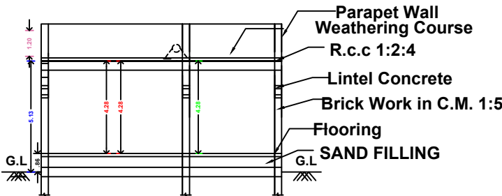
SECTION ON "BB"
