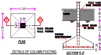
DETAILS OF COLUMN FOOTING
