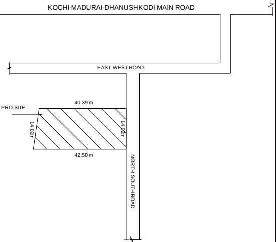
TOPO PLAN
