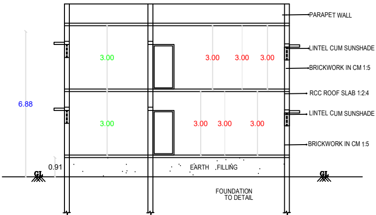
SECTION AB
