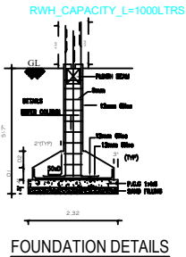
FOUNDATION DETAILS
