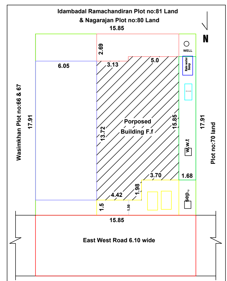
SITE PLAN CUM KEYPLAN
