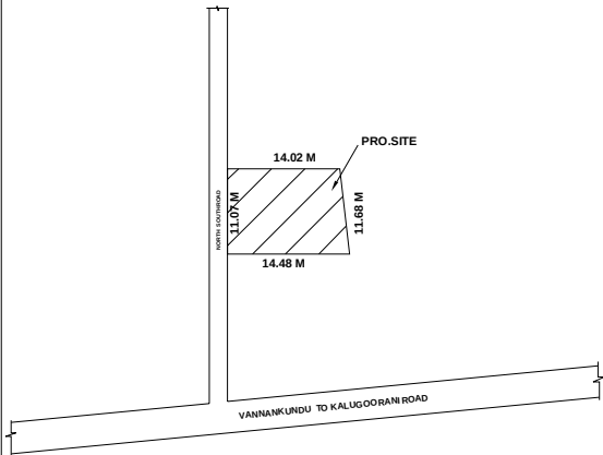
TOPO PLAN
