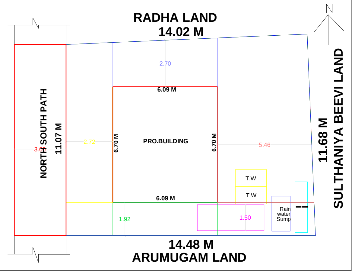
SITE FLOOR PLAN PROPOSED
